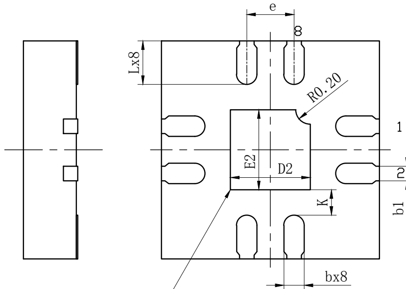
BOTTOM VIEW
