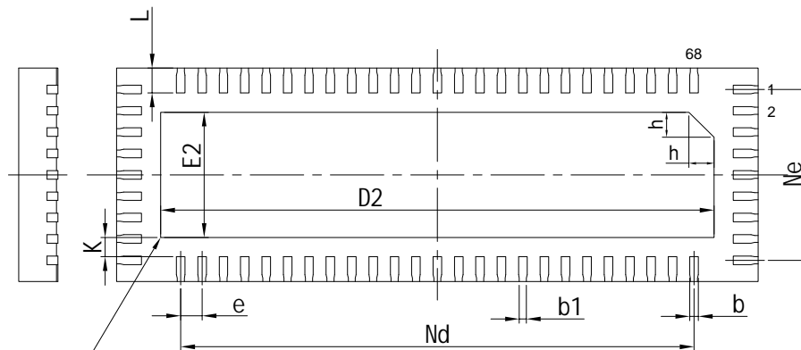
BOTTOM VIEW
