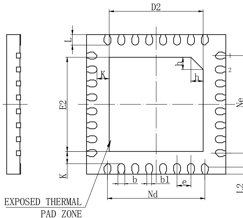
BOTTOM VIEW
