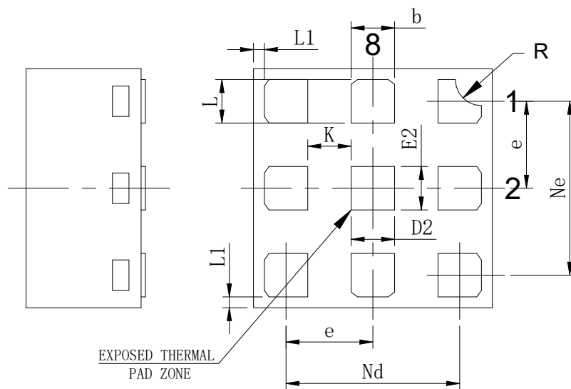
BOTTOM VIEW
