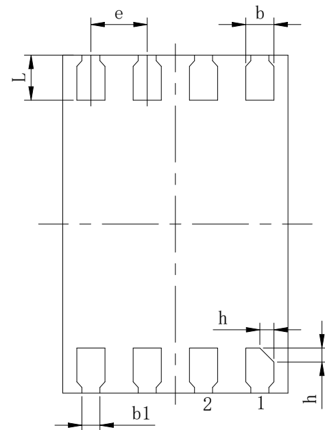
BOTTOM VIEW
