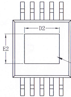
BOTTOM VIEW
